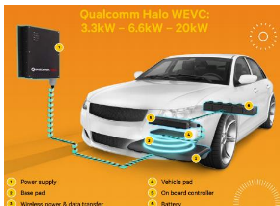
Figure 34 – Wireless Charging
