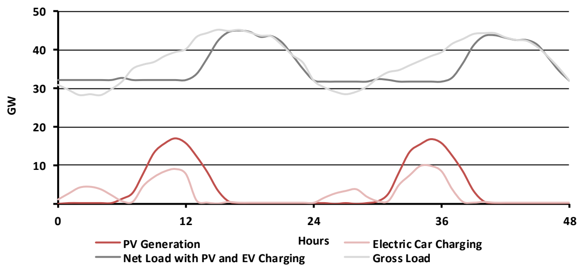
Figure 21 – Managed Solar PV Interactions
